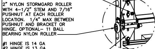
DETAIL B
