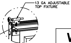
LOW HEADROOM TRACK DETAIL F
