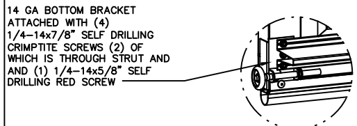
DETAIL D
